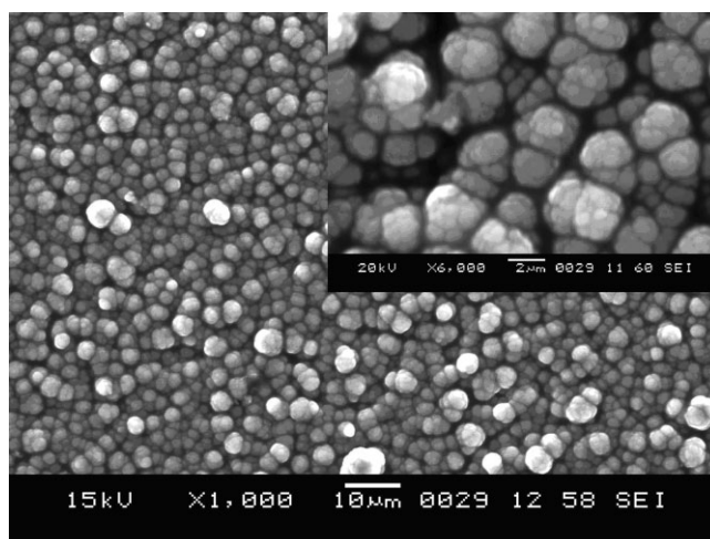
Figure 13 SEM image of PPy/SS electrode surface prepared at 0.01M SDS concentration (inset: magnified view of the surface).
